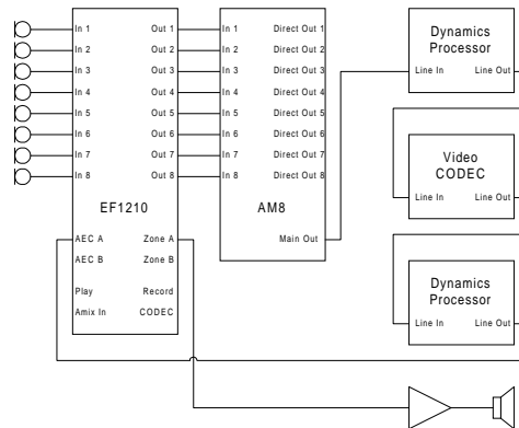
Figure 4: Recommended placement of an external dynamics processor in an EF1210 system.
