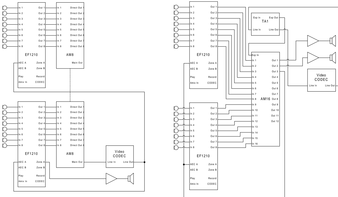
Figure 1a: EF1210 and AM8 without sound reinforcement. Figure 1b: EF1210 and AM16 with sound reinforcement.
