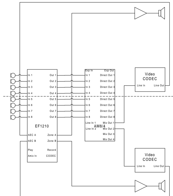
Figure 2: Using the EF1210 with one AM8/4 for two different rooms.
